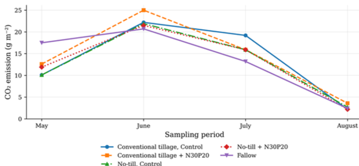
Figure 4. Seasonal dynamics of soil CO 2 emissions under different tillage systems and mineral fertilization levels in 2025
