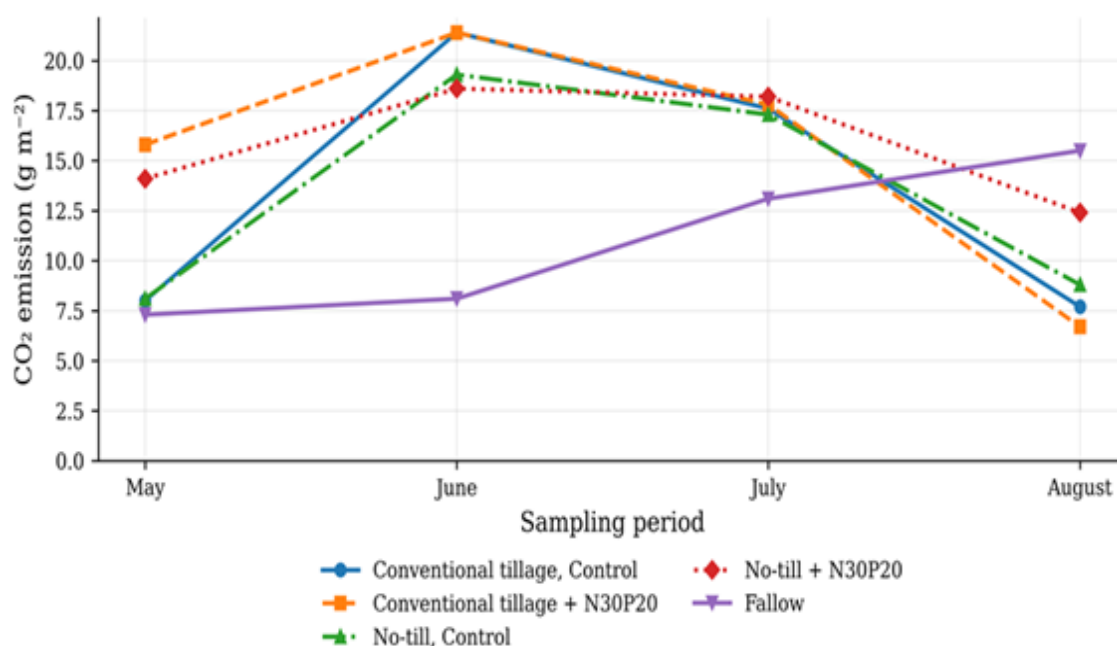
Figure 3. Seasonal dynamics of soil CO_2 emissions under different tillage systems and mineral fertilization levels in 2024
