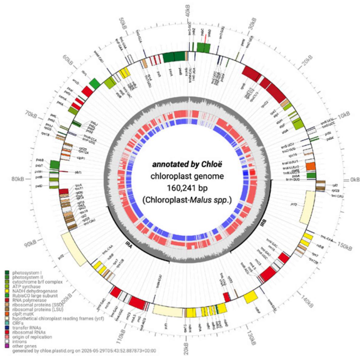
Figure 1. Gene structure in the Malus spp. chloroplast genome
