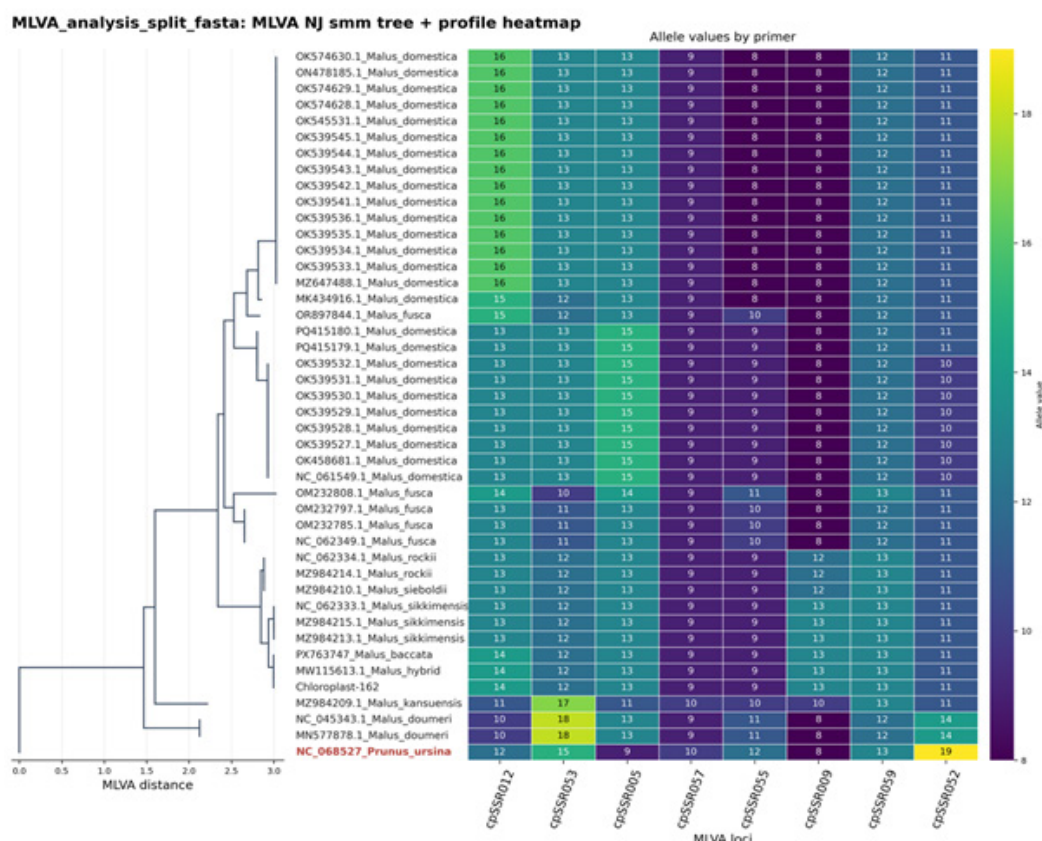
Figure 3. cpSSR/VNTR marker matrix for 44 samples of the genera Malus and Prunus
