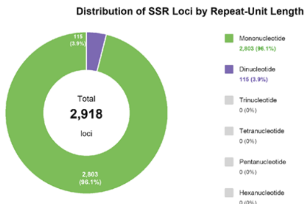
Figure 2. Distribution of SSR loci identified in Malus chloroplast genomes by monomer length
